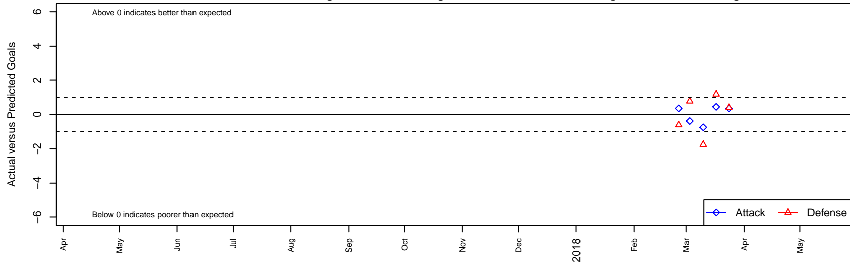
Irish America G04 Dots are actual minus expected GF (blue circles) and GA (red triangles). Blue line is smoothed change in attack strength. Red is smoothed change in defense strength.
